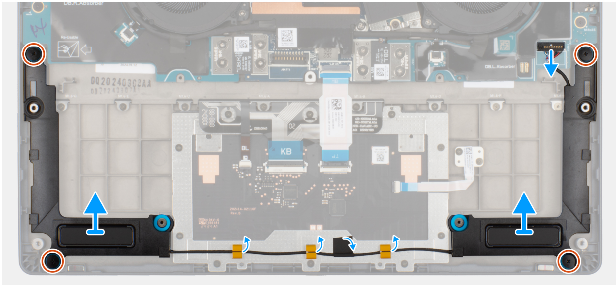
Figure 34. Removing the speakers without antenna (WLAN configuration)
